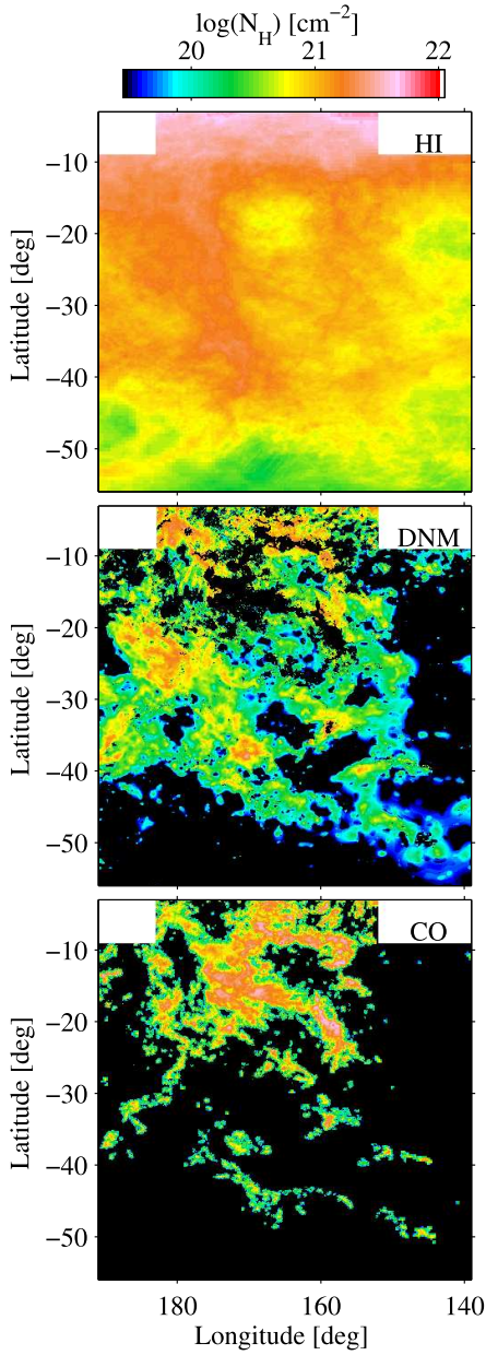
Fig. 5. Hydrogen column density maps, N_{\text{H}} , in the HI, DNM, and CO-bright phases, obtained for an HI spin temperature of 400 K. The N_{\text{H}} map in the DNM is based on the dust residuals over the HII, HI, and CO expectations and on the average the \tau_{353}/N_{\text{H}} opacity measured in \gamma rays in this phase. The N_{\text{H}} map in the CO phase uses the X_{\text{CO}} factors measured in \gamma rays for each cloud.
