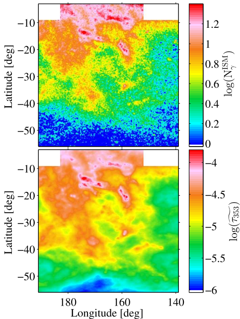
Fig. 2. Top : \gamma -ray count of gaseous origin in the 10^{2.6} - 10^5 MeV energy band. The map was constructed by subtracting the point sources and ancillary, non-gaseous, components from the data. Bottom : dust optical depth processed through the LAT IRFs.
