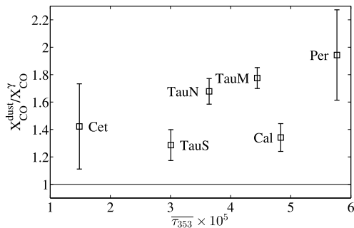
Fig. 4. Evolution of the ratio between the dust and \gamma -ray measurements of X_{\text{CO}} in the different clouds as a function of the average dust optical depth, \tau_{353} , in the cloud.
