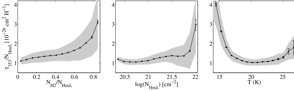
Fig. 8. Evolution of the dust opacity as a function of the molecular fraction in the gas column ( left ), the total gas column density N_{\text{Hm}\lambda} ( middle ), and the dust color temperature ( right ). To estimate the molecular fraction in N_{\text{H}} , the DNM is assumed to be 50% molecular. The error bars and shaded areas give the standard error on the mean and standard deviation in each bin.
