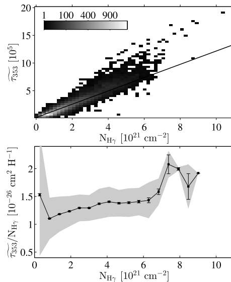
Fig. 7. Top: 2D histograms of the correlations between the total gas column density, N_{\text{H}\gamma} , measured with the 0.4-100 GeV interstellar \gamma rays, and the dust optical depth convolved with the LAT response. Bottom: evolution of the dust opacity in equally spaced bins in N_{\text{H}\gamma} . The error bars and shaded areas give the standard error on the mean and standard deviation in each bin.
