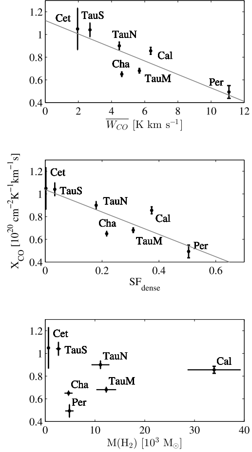
Fig. 3. Evolution of the X_{\text{CO}} factor in the different clouds as measured in \gamma rays in the total energy band. The evolution is displayed with the average CO intensity, \overline{W_{\text{CO}}} , measured in a cloud above 1 K km s -1 (top), with the surface fraction, \text{SF}_{\text{dense}} , of the dense cores (see Eq. 1) (middle), and with the H 2 mass found in the CO-bright phase of the clouds (bottom). The Chamaeleon data comes from Planck and Fermi Collaborations (2014).
