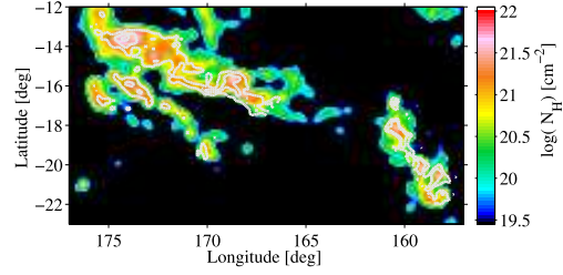
Fig. 6. Hydrogen column density map, N_{\text{H}} , of additional gas obtained in the ^{12}\text{CO} -saturated part of the Taurus and Perseus clouds, and overlaid with the ^{13}\text{CO} contours at 2 and 4 K \text{km s}^{-1} from Narayanan et al. (2008); Ridge et al. (2006).
