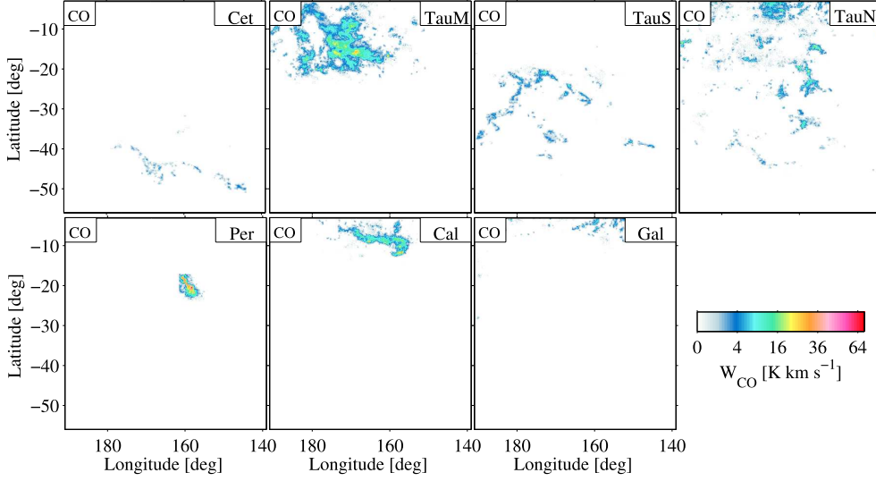
Fig. 1. Integrated CO intensity W_{\text{CO}} , in square-root scale, for the Cetus, Main Taurus, South Taurus, North Taurus, Perseus, and California clouds and the Galactic disc background.
